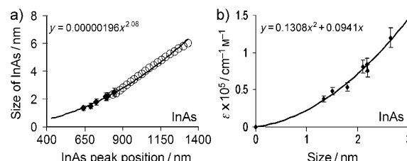
Figure 4. TEM and AA results for several InAs/CdSe core-shell samples (top). a) Size of InAs nanocrystals versus their first excitonic absorption peak ( \circ literature, \blacklozenge this work). b) The molar extinction coefficient ( \epsilon ) of InAs nanocrystals. The solid lines in (a) and (b) are numerical fittings.
